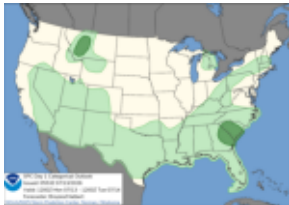
SPC Convective Outlook
