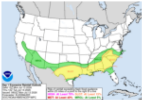
WPC Excessive Rainfall Outlook
